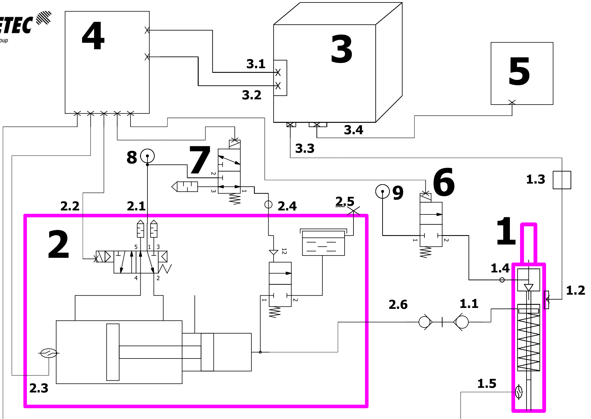
RIVETEC HHTC60 + RHP P2 + KRB 010 Connection Diagram
